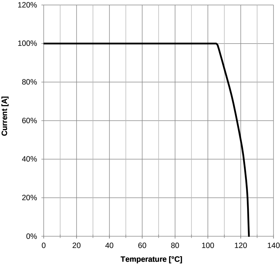
Derating Curve:
