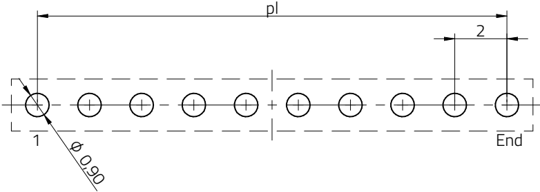
Recommended P.C.B Layout General tolerance \pm 0.05
