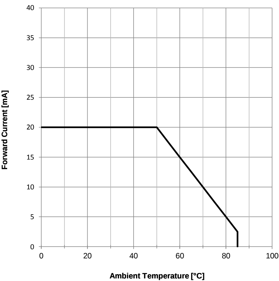
Derating Curve:
