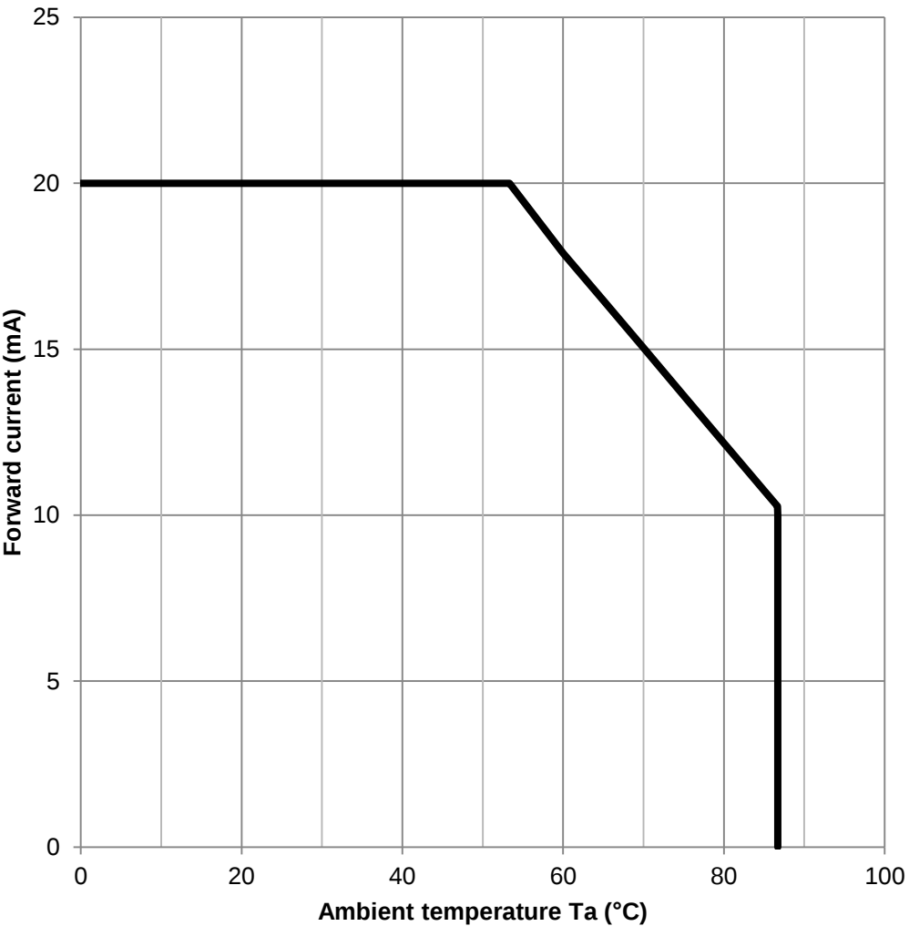
Derating Curve:
