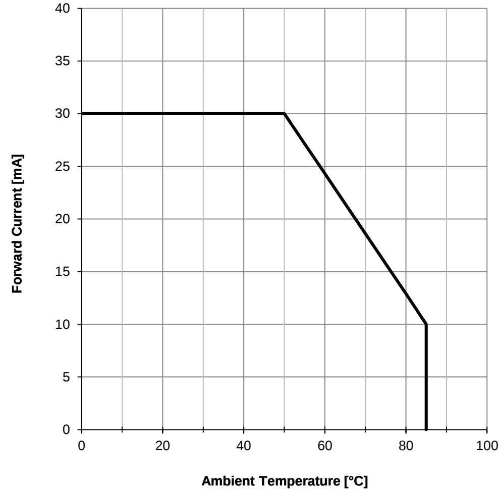
Derating Curve:
