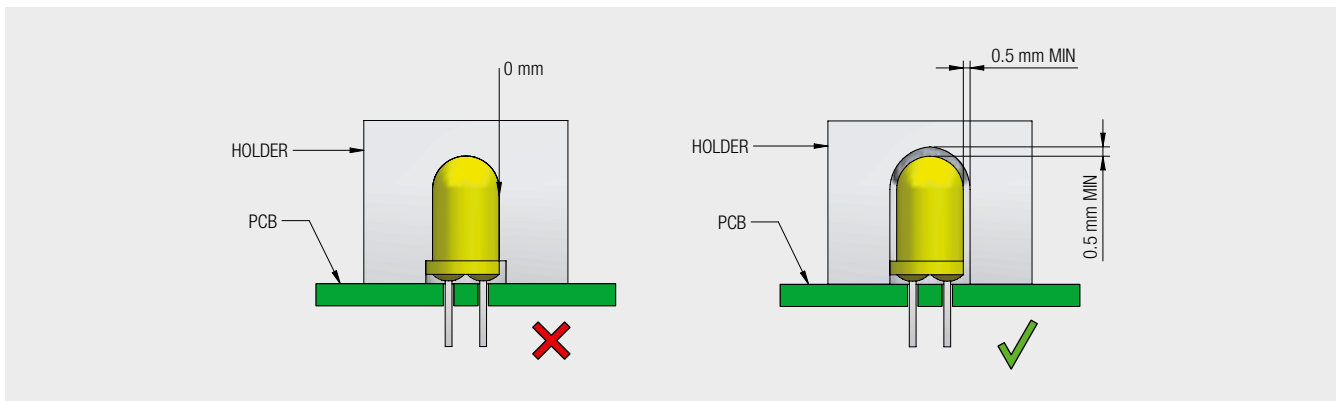
Figure 33: After soldering
