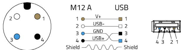
Figure 9 - M12 A-Coded plug to USB 2.0 pinout
