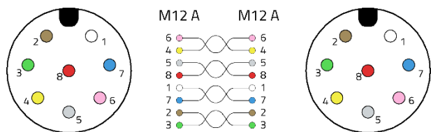
Figure 3 - 10BASE-T M12 to M12 pin assignment
