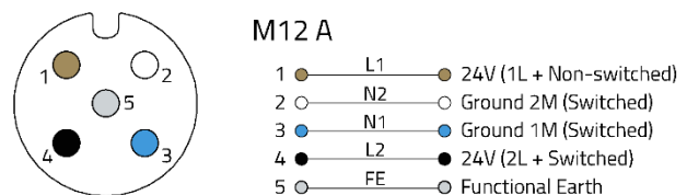
Figure 13 - PROFIBUS Pin assignment for 5-pin M12 A-Coded receptacle
