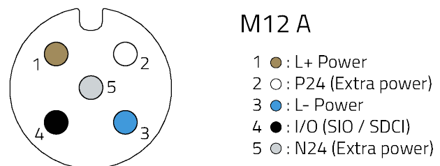
Figure 7 - Class B ports and cables on Hub and Device sides will be 5-pin M12 A-Coded receptacles
