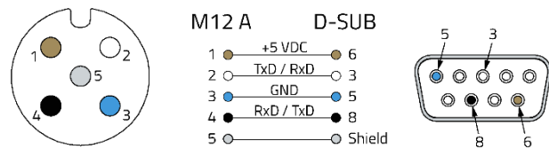
Figure 12 - RS-485 pinout at M12 A-coded receptacle
